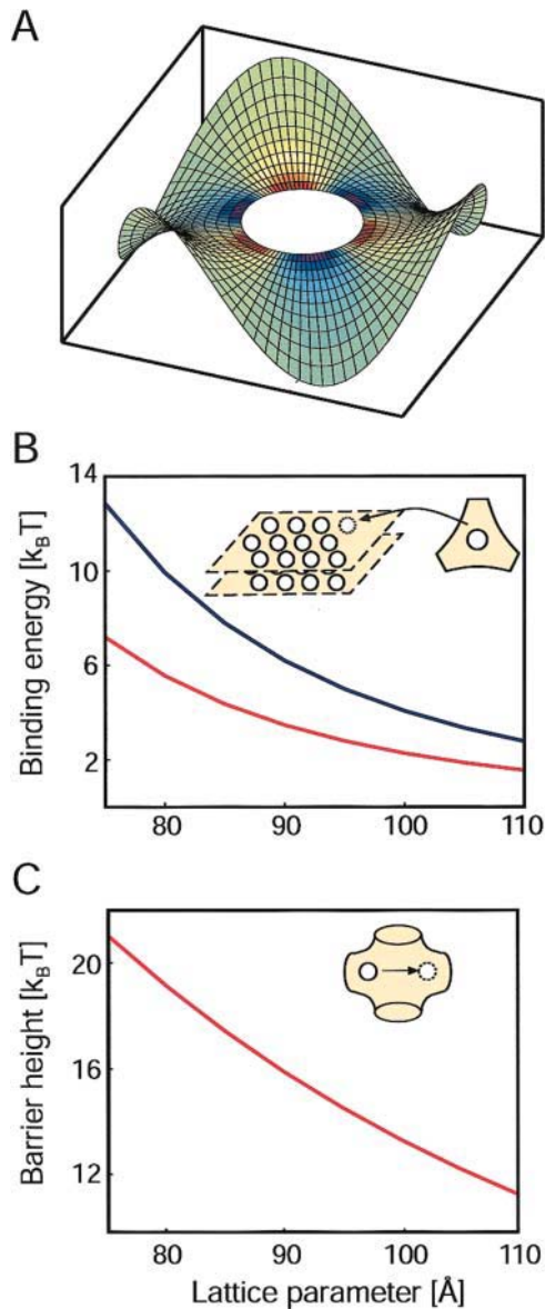
FIGURE 3 Protein energetics in the Pn3m cubic phase. (A) Computed deformation field of the monkey saddle region with a single inclusion in the bulk Pn3m cubic phase. The surface color (red and blue) represents the induced mean curvature radiating outward from the inclusion. (B) Binding energy for adding a single bR-sized protein to a growing lamellar crystal as a function of the lattice parameter. The energy is plotted using an upper and a lower bilayer bending modulus determined from experimentally measured monolayer bending moduli for the monoolein system. The monolayer values are \kappa_m = 2.8 k_B T (Vacklin et al., 2000), corresponding to the red curve, and \kappa_m = 5.0 k_B T (Chung and Caffrey, 1994), corresponding to the blue curve. These curves are plotted with bilayer bending moduli twice the recorded monolayer values. This assumes no interdigitation between the monolayer leaflets and is likely an underestimate of the true bilayer bending modulus. The elastic energy increases sharply at smaller lattice parameters, which drives the formation of crystals. (C) The energy barrier for crossing from one minimum energy site to the next is plotted as a function of the lattice parameter. The bilayer bending modulus corresponding to Vacklin et al.'s monolayer value was used (Vacklin et al., 2000). This barrier to diffusion slows the movement of proteins in the cubic phase.
